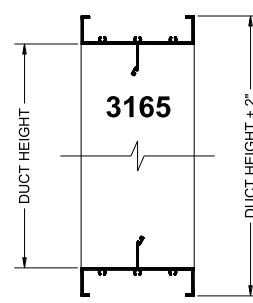
3165 – Flanged-to-Duct
