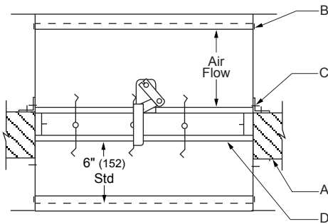
Horizontal Mount (Single Side Mounting Angle)
