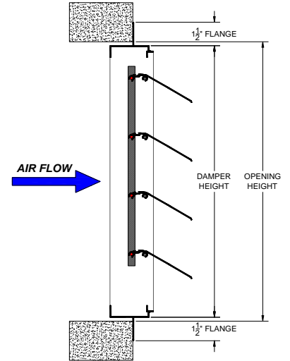
FFM FRONT FLANGE MOUNT
