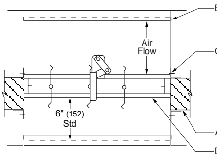
Horizontal Mount (2-sided Mounting Angles)
